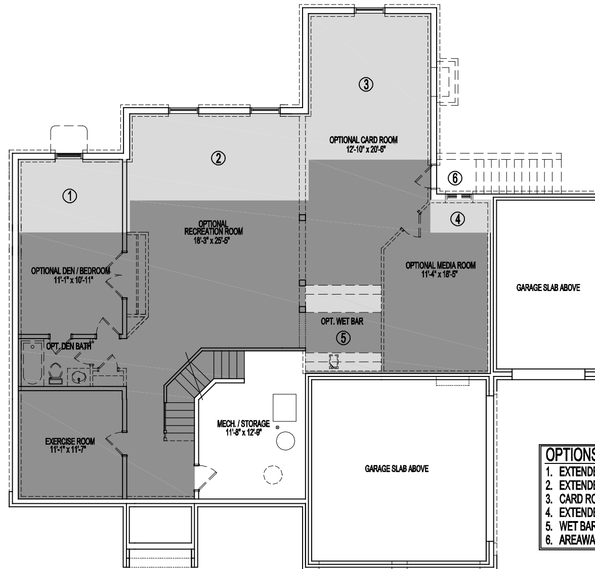
FOUNDATION / BASEMENT PLAN
