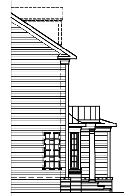
PARTIAL LEFT SIDE ELEVATION ELEVATION #1E W/ BAY WINDOW 01-18-18
