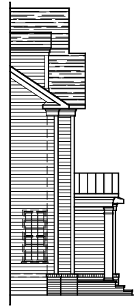
PARTIAL LEFT SIDE ELEVATION ELEVATION #5A 01-18-18
