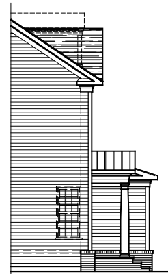
PARTIAL LEFT SIDE ELEVATION ELEVATION #2A 01-18-18
