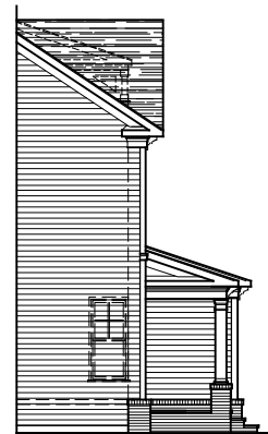
PARTIAL LEFT SIDE ELEVATION ELEVATION #3B 01-18-18
