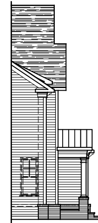
PARTIAL LEFT SIDE ELEVATION ELEVATION #7A 01-18-18
