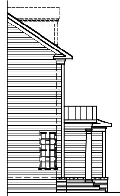
PARTIAL LEFT SIDE ELEVATION ELEVATION #1A 01-18-18
