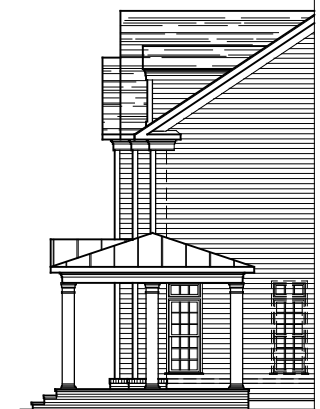
PARTIAL RIGHT SIDE ELEVATION ELEVATION #6C 1-16-18
