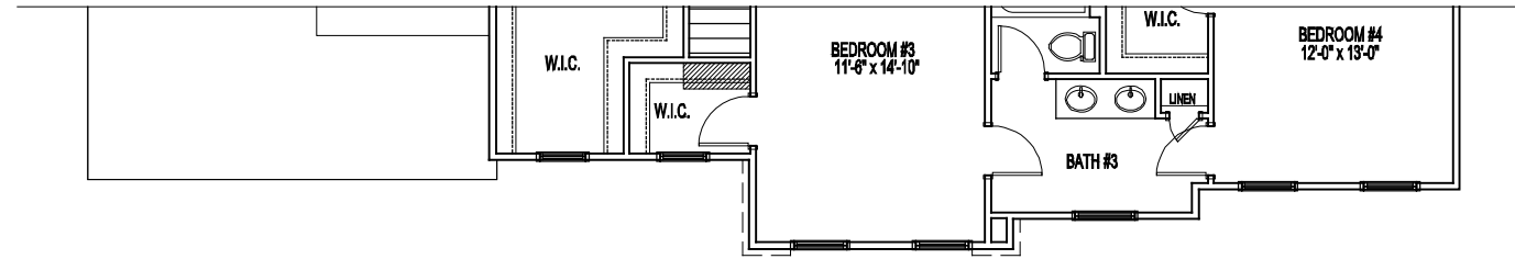
PARTIAL SECOND FLOOR PLAN ELEVATION 6A
