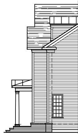
RIGHT SIDE ELEVATION ELEVATION #10A 1-16-18
