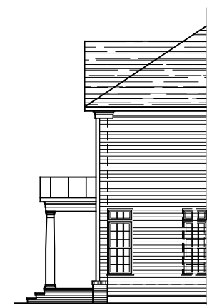
PARTIAL RIGHT SIDE ELEVATION ELEVATION #4A 1-16-18
