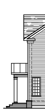
PARTIAL RIGHT SIDE ELEVATION ELEVATION #1A 1-16-18
