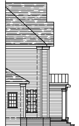
PARTIAL LEFT SIDE ELEVATION ELEVATION #6A 01-17-18
