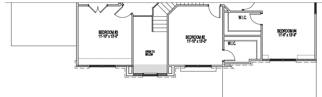
PARTIAL SECOND FLOOR PLAN ELEVATION #7A & 7B 01-17-18
