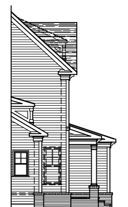
PARTIAL LEFT SIDE ELEVATION ELEVATION #3B 01-17-18
