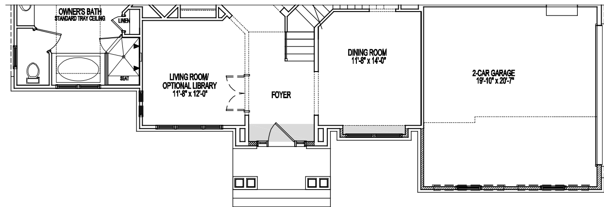
PARTIAL FIRST FLOOR PLAN ELEVATION #7A 01-17-18
