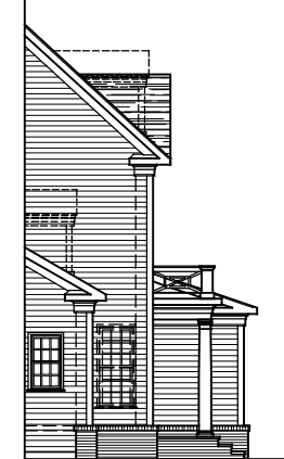
PARTIAL LEFT SIDE ELEVATION ELEVATION #2B 01-17-18
