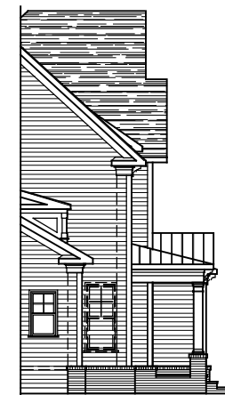
PARTIAL LEFT SIDE ELEVATION ELEVATION #7B 01-17-18
