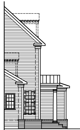
PARTIAL LEFT SIDE ELEVATION ELEVATION #1A 01-17-18
