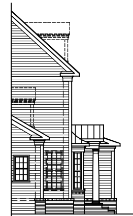
PARTIAL LEFT SIDE ELEVATION ELEVATION #1E W/ PORTICO W/ BAY 01-17-18
