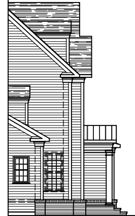
PARTIAL LEFT SIDE ELEVATION ELEVATION #5A 01-17-18
