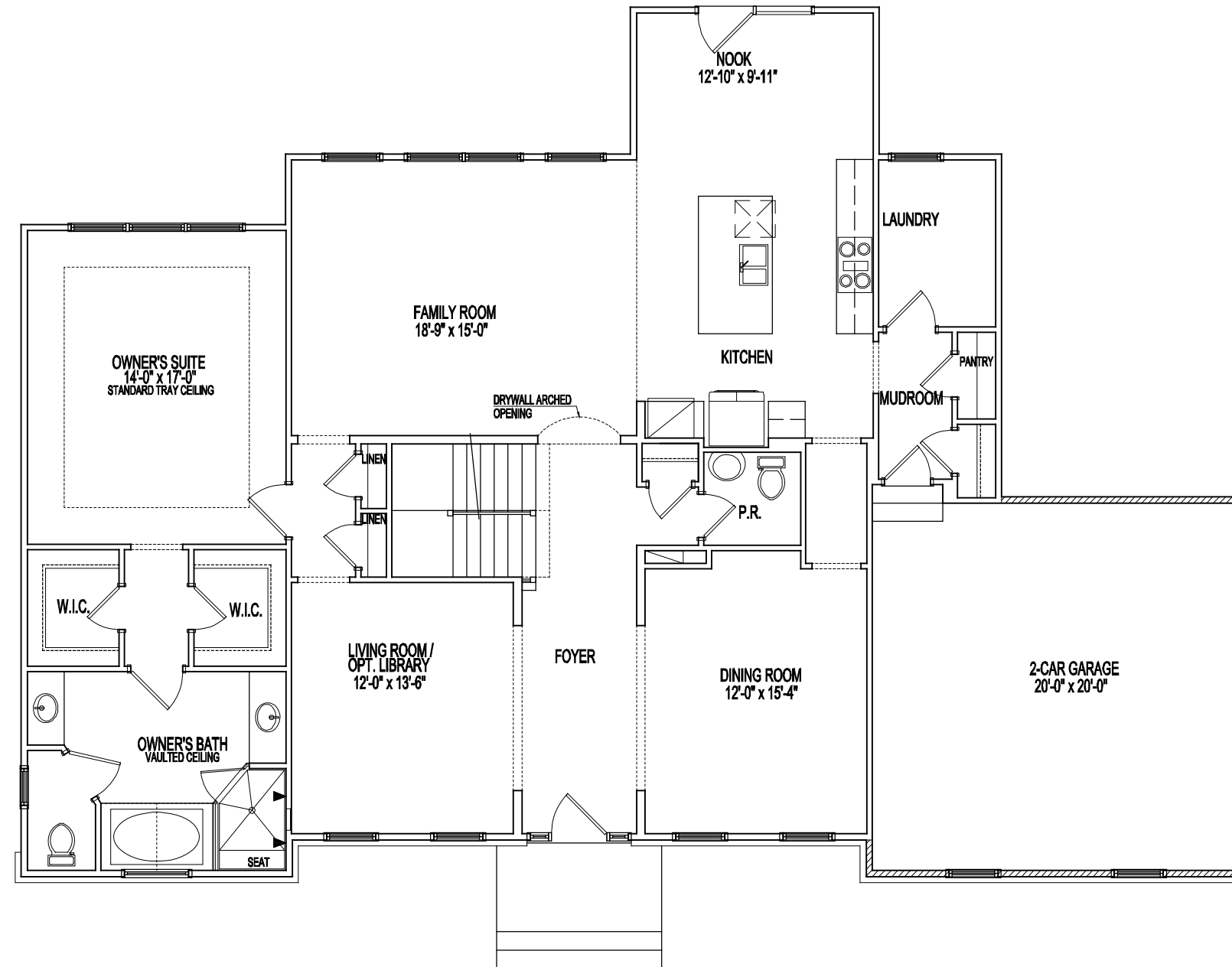
STANDARD FIRST FLOOR PLAN
