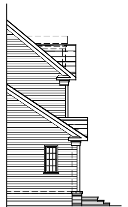
PARTIAL FRONT ELEVATION ELEVATION #3A 01-18-18
