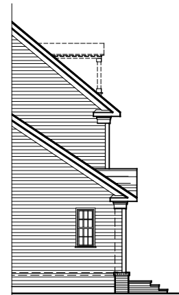
PARTIAL FRONT ELEVATION ELEVATION #1A 01-18-18
