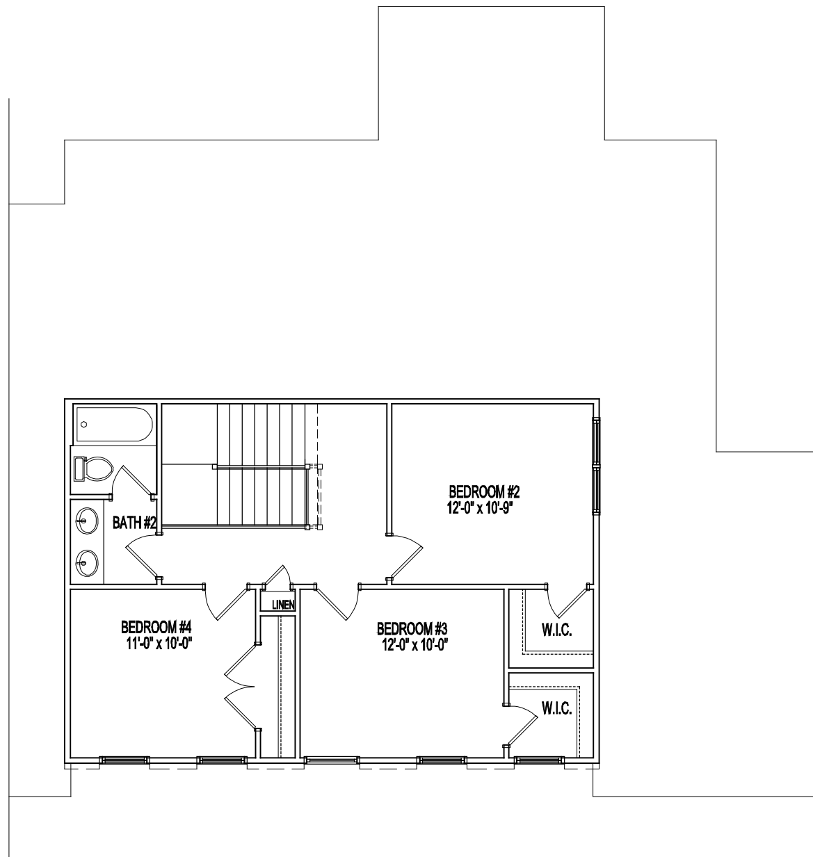
STANDARD SECOND FLOOR PLAN
