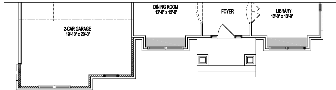
PARTIAL FIRST FLOOR PLAN ELEVATION #7A & 8A 11-15-2018
