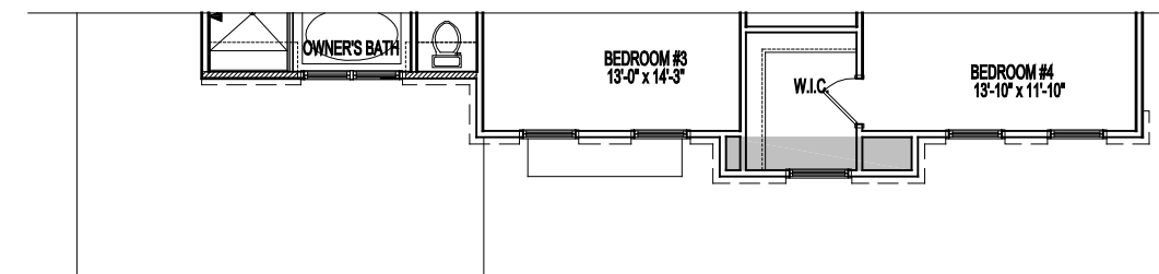
PARTIAL SECOND FLOOR PLAN ELEVATION #5A & 5B 11-15-2018
