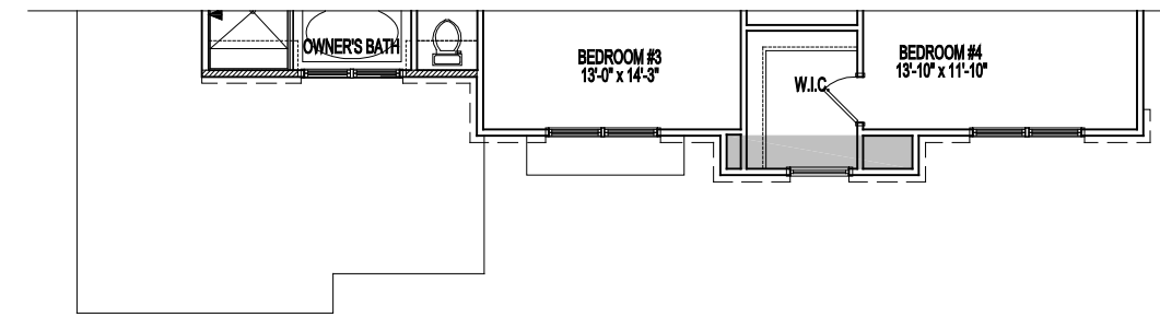
PARTIAL SECOND FLOOR PLAN ELEVATION #4 & 4A 11-15-2018
