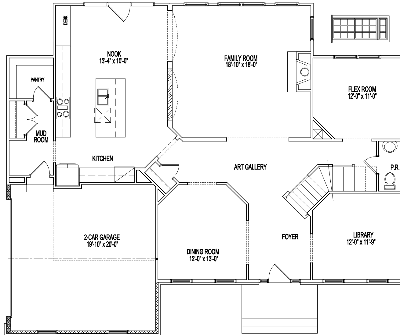
STANDARD FIRST FLOOR PLAN
