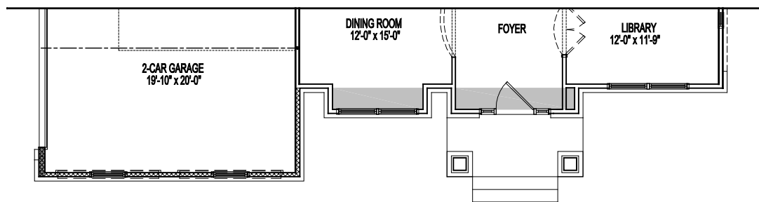
PARTIAL FIRST FLOOR PLAN ELEVATION #5A 11-15-2018
