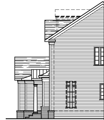
PARTIAL RIGHT ELEVATION ELEVATION #8A 11-15-2018
