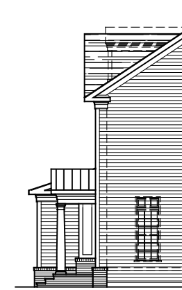
PARTIAL RIGHT ELEVATION ELEVATION #2A 11-15-2018
