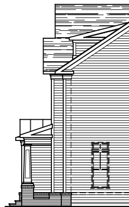
PARTIAL RIGHT ELEVATION ELEVATION #5A 11-15-2018
