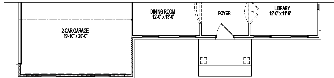
PARTIAL FIRST FLOOR PLAN ELEVATION #9A 11-15-2018
