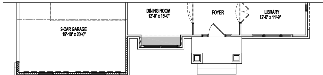
PARTIAL FIRST FLOOR PLAN ELEVATION #3A 11-15-2018
