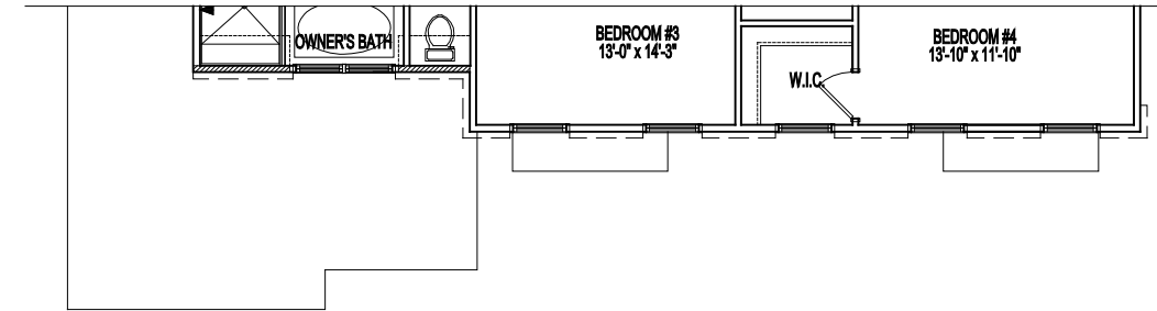
PARTIAL SECOND FLOOR PLAN ELEVATION #7A & 8A 11-15-2018
