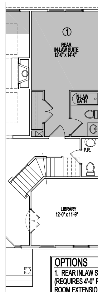
PARTIAL FIRST FLOOR PLAN
