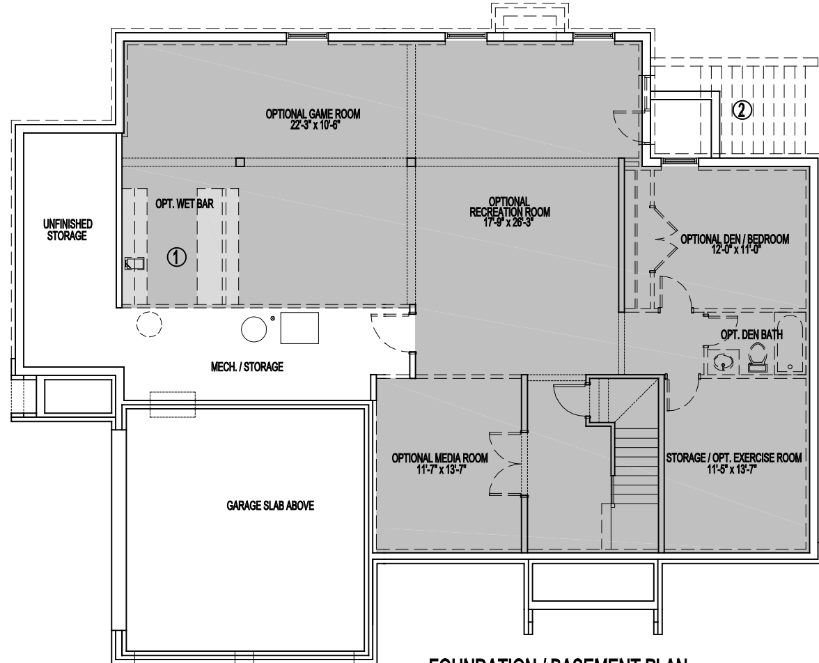
FOUNDATION / BASEMENT PLAN OPTIONS 1. WET BAR 2. DOUBLE WIDE AREAWAY 08-29-19
