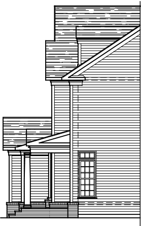
FRONT ELEVATION ELEVATION #12B
