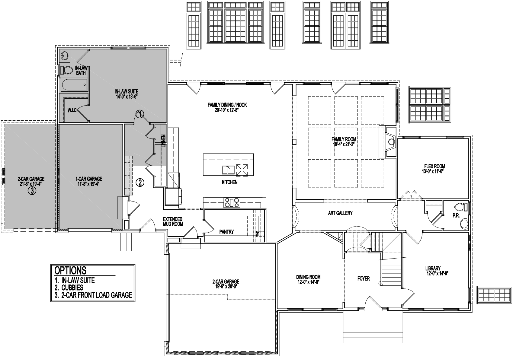
FIRST FLOOR PLAN (REQUIRES EXTENDED MUD ROOM) 08-29-19 (REQUIRES 1-CAR FRONT LOAD GARAGE)
