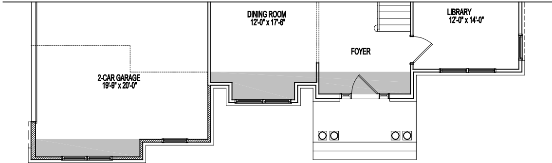
PARTIAL FIRST FLOOR PLAN ELEVATION 11A 08-29-19
