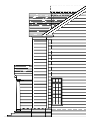
PARTIAL RIGHT SIDE ELEVATION ELEVATION #13A 08-29-19
