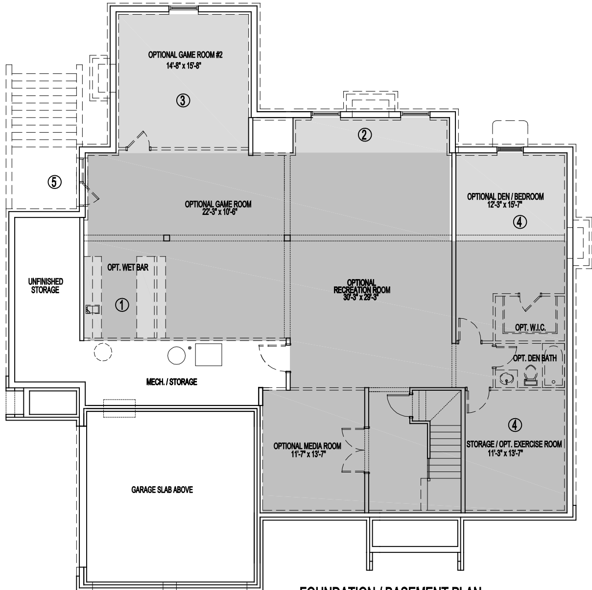
FOUNDATION / BASEMENT PLAN OPTIONS 1. WET BAR 2. EXTENDED REC ROOM 3. GAME ROOM #2 4. OPT. DEN / BEDROOM 5. DOUBLE WIDE AREAWAY 08-29-19
