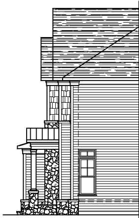
PARTIAL RIGHT SIDE ELEVATION
