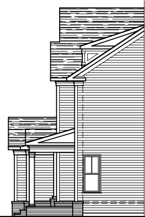
FRONT ELEVATION ELEVATION #11B 08-29-19
