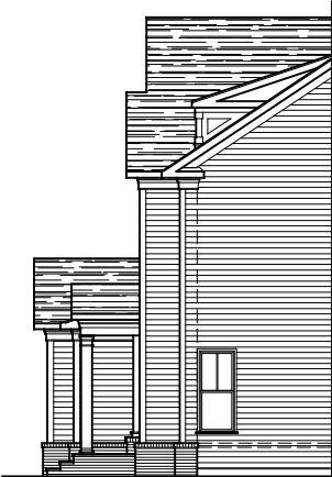
PARTIAL RIGHT SIDE ELEVATION ELEVATION #11A 08-29-19
