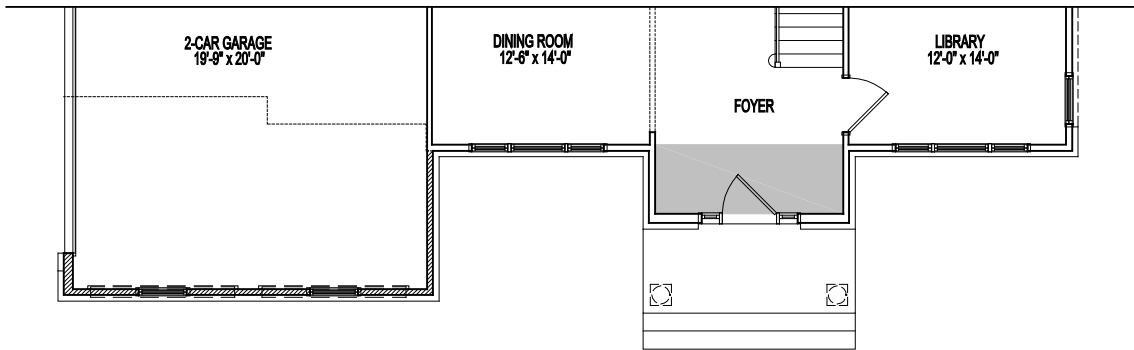
PARTIAL FIRST FLOOR PLAN ELEVATION 13, 13A 08-29-19
