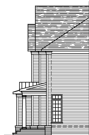
PARTIAL RIGHT SIDE ELEVATION ELEVATION #3B 08-29-19
