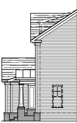
PARTIAL RIGHT ELEVATION ELEVATION #3A 08-29-2019
