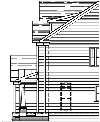
PARTIAL RIGHT ELEVATION ELEVATION #5A 08-29-2019
