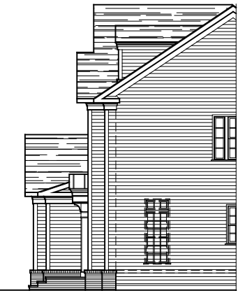
PARTIAL RIGHT ELEVATION ELEVATION #4A 08-29-2019
