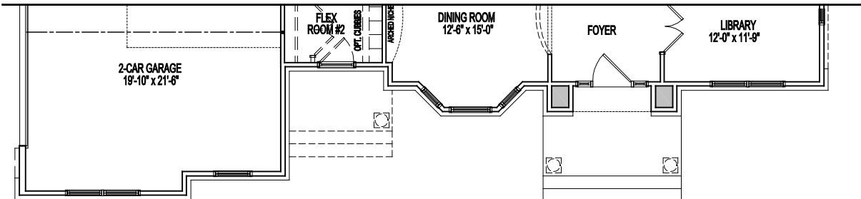
PARTIAL FIRST FLOOR PLAN ELEVATION #4 & 4A 08-29-2019
