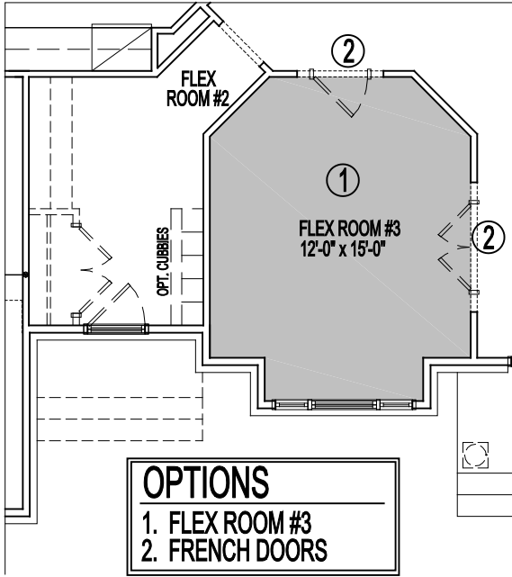
PARTIAL FIRST FLOOR PLAN
