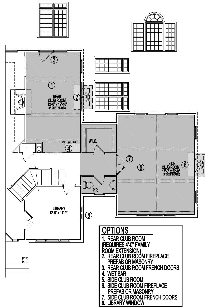
PARTIAL FIRST FLOOR PLAN
