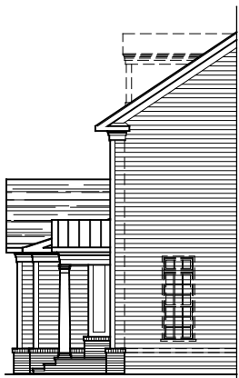
PARTIAL RIGHT ELEVATION ELEVATION #1A 08-29-2019
