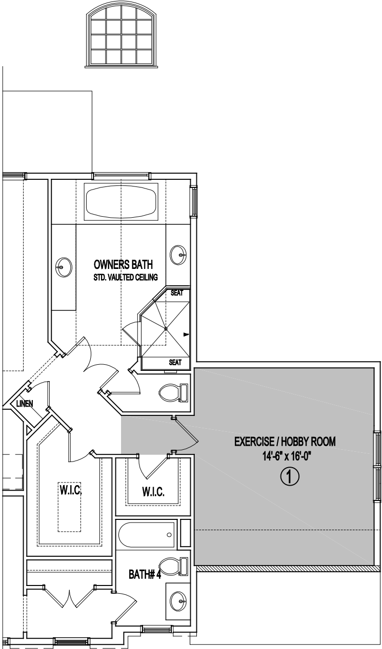
PARTIAL SECOND FLOOR PLAN
