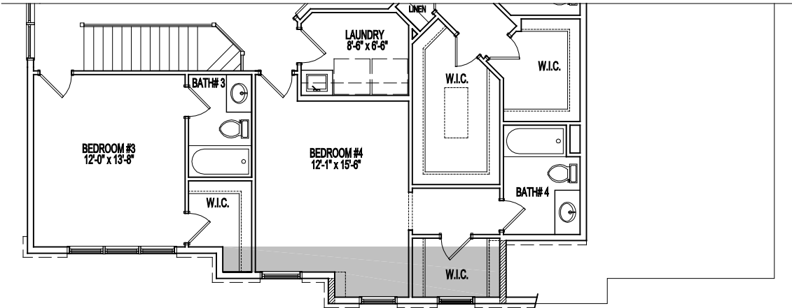
PARTIAL SECOND FLOOR PLAN ELEVATION #4A & 4B 08-29-19
