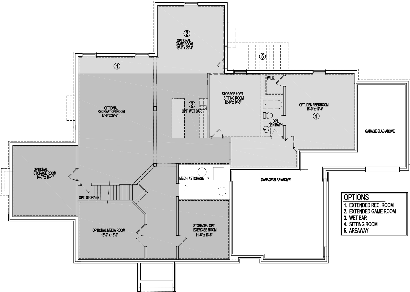
FOUNDATION / BASEMENT PLAN 08-29-19
