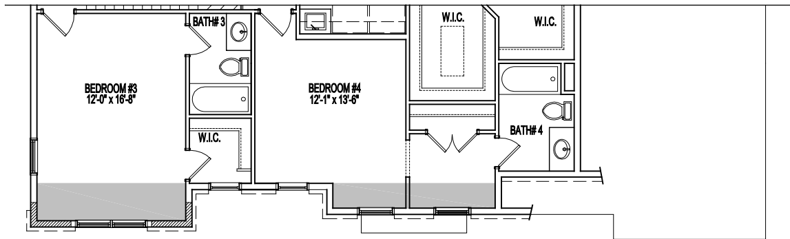
PARTIAL SECOND FLOOR PLAN ELEVATION #5A 08-29-19
