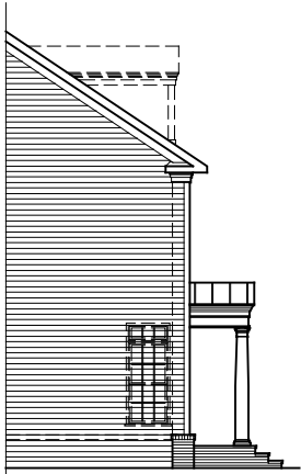
PARTIAL LEFT SIDE ELEVATION ELEVATION #1A 08-29-19
