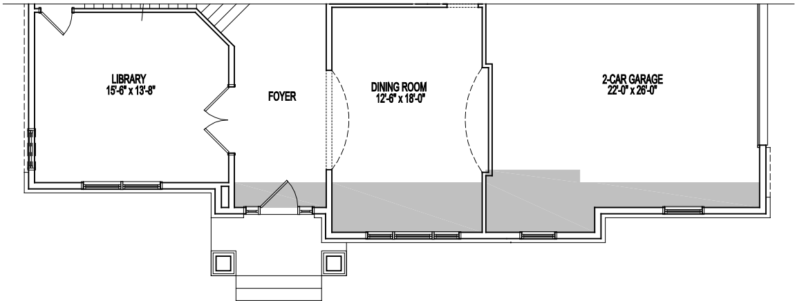
PARTIAL FIRST FLOOR PLAN ELEVATION #4A & 4B 08-29-19
