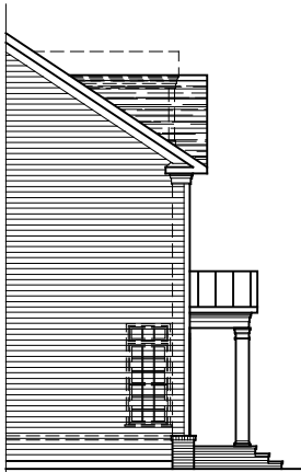
PARTIAL LEFT SIDE ELEVATION ELEVATION #2A 08-29-19
