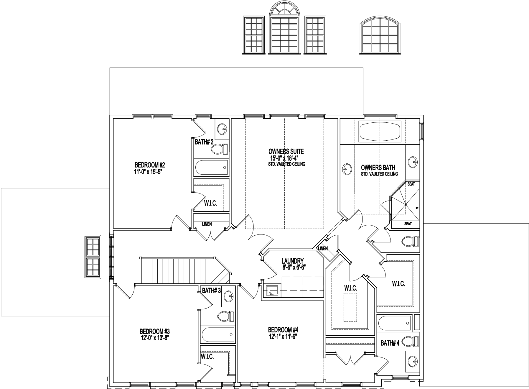
STANDARD SECOND FLOOR PLAN
