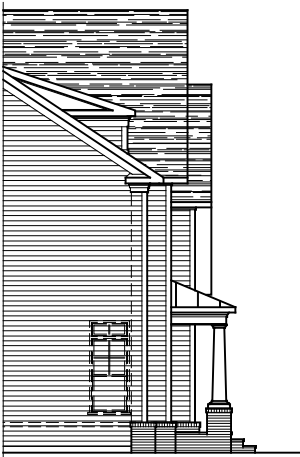
PARTIAL LEFT SIDE ELEVATION ELEVATION #4A 08-29-19
