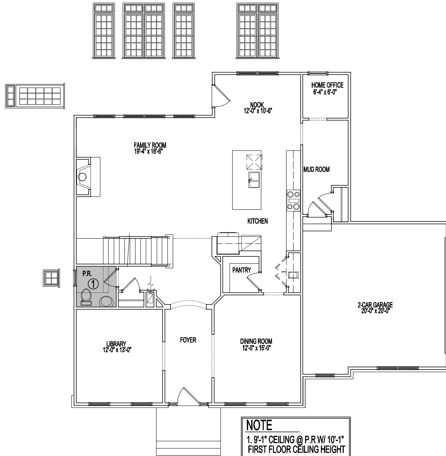
STANDARD FIRST FLOOR PLAN
