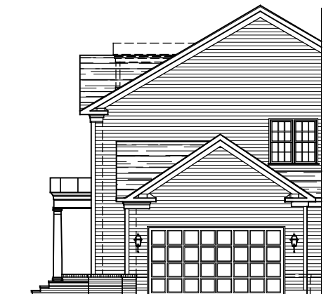
PARTIAL RIGHT SIDE ELEVATION ELEVATION #2A 05-18-20
