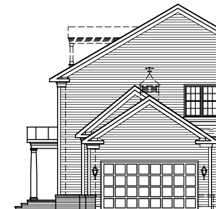
PARTIAL RIGHT SIDE ELEVATION ELEVATION #1A 05-18-20
