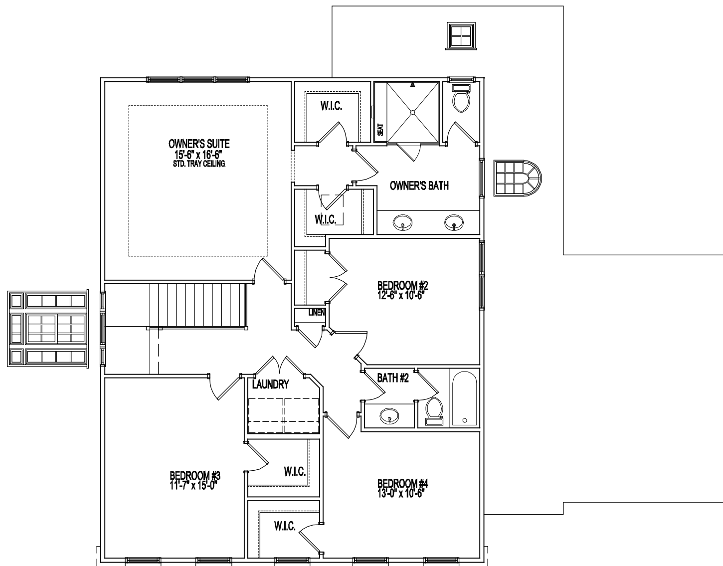
STANDARD SECOND FLOOR PLAN
