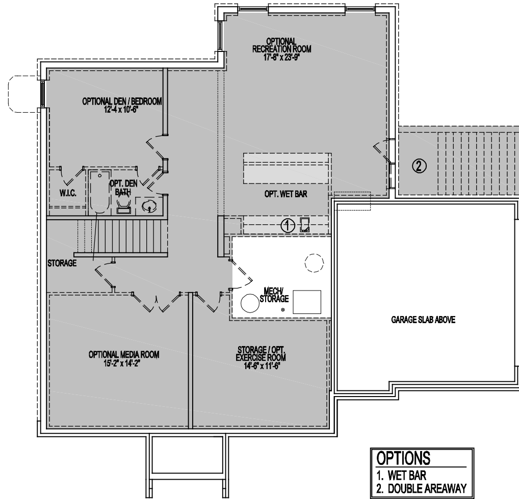
FOUNDATION / BASEMENT PLAN
