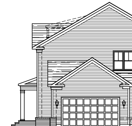
PARTIAL RIGHT SIDE ELEVATION ELEVATION #8A 05-18-20
