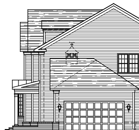
PARTIAL RIGHT SIDE ELEVATION ELEVATION #4B 05-18-20
