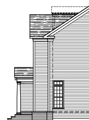
PARTIAL RIGHT SIDE ELEVATION ELEVATION #13A 04-23-20
