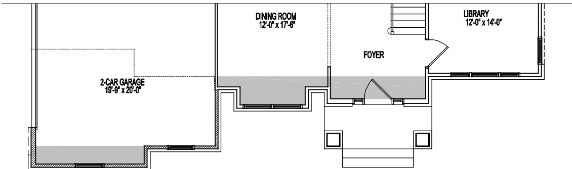
PARTIAL FIRST FLOOR PLAN ELEVATION 10A 04-23-20
