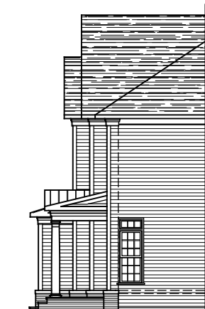
PARTIAL RIGHT SIDE ELEVATION ELEVATION #3B 04-23-20
