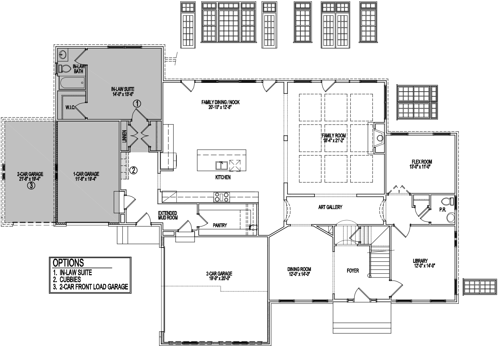
FIRST FLOOR PLAN (REQUIRES EXTENDED MUD ROOM) 04-23-20 (REQUIRES 1-CAR FRONT LOAD GARAGE)
