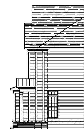
PARTIAL RIGHT SIDE ELEVATION ELEVATION #3A 04-23-20
