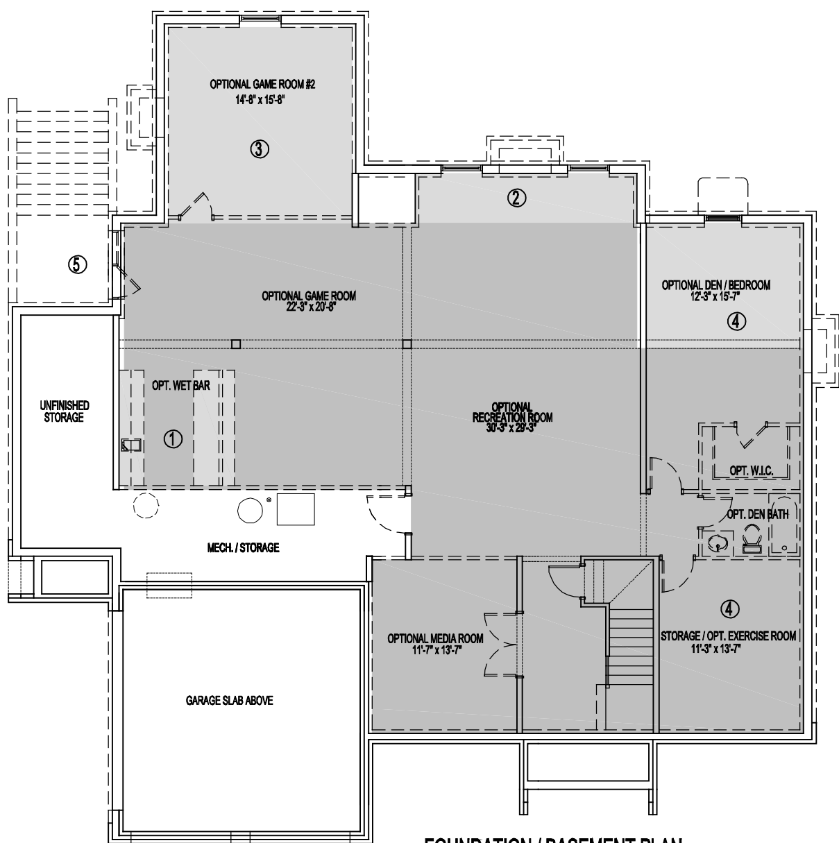
FOUNDATION / BASEMENT PLAN OPTIONS 1. WET BAR 2. EXTENDED REC ROOM 3. GAME ROOM #2 4. OPT. DEN / BEDROOM 5. DOUBLE WIDE AREAWAY 04-23-20
