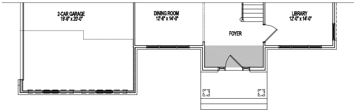
PARTIAL FIRST FLOOR PLAN ELEVATION 13, 13A 04-23-20
