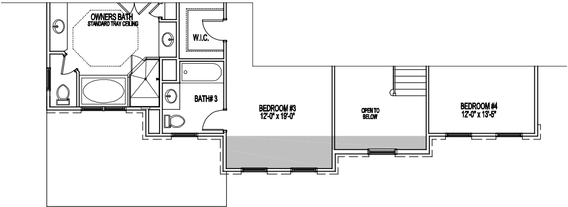
PARTIAL UPPER FLOOR PLAN ELEVATION 3A, 3B 04-23-20
