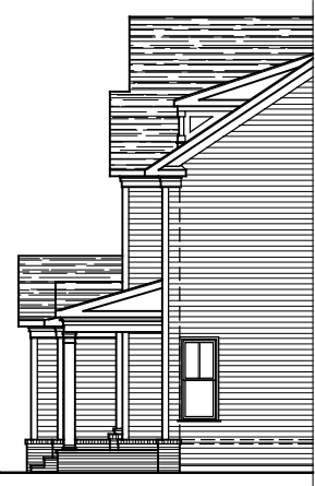
FRONT ELEVATION ELEVATION #11B 04-23-20
