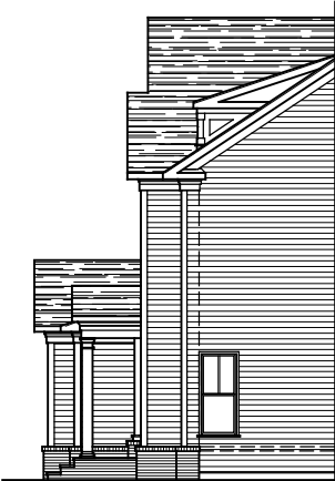
PARTIAL RIGHT SIDE ELEVATION ELEVATION #11A 04-23-20
