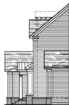
PARTIAL LEFT ELEVATION ELEVATION #1A 08-29-19
