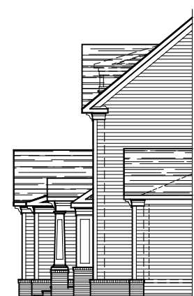
PARTIAL LEFT ELEVATION ELEVATION #1A 08-29-19
