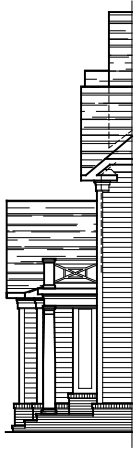
PARTIAL LEFT ELEVATION ELEVATION #5B 08-29-19
