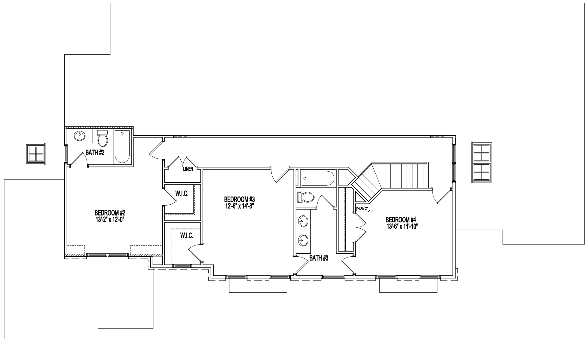
STANDARD UPPER FLOOR PLAN
