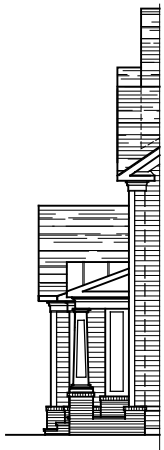
PARTIAL RIGHT ELEVATION ELEVATION #10B 08-29-2019
