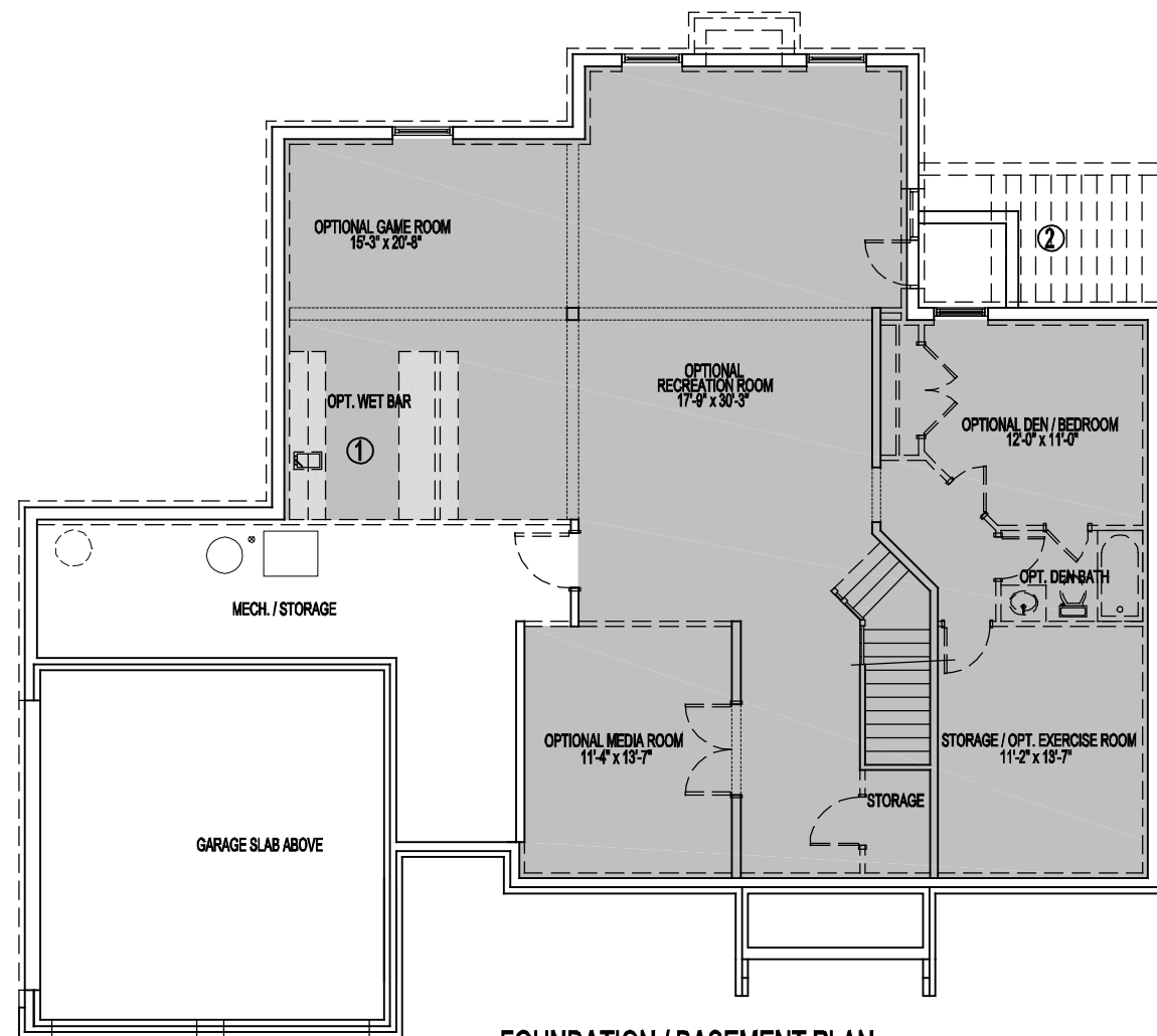
FOUNDATION / BASEMENT PLAN
