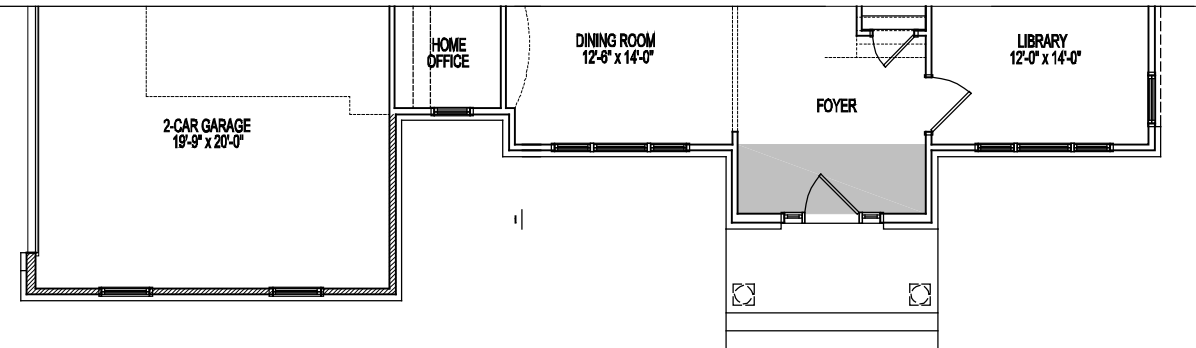
PARTIAL FIRST FLOOR PLAN ELEVATION 13, 13A 01-13-20
