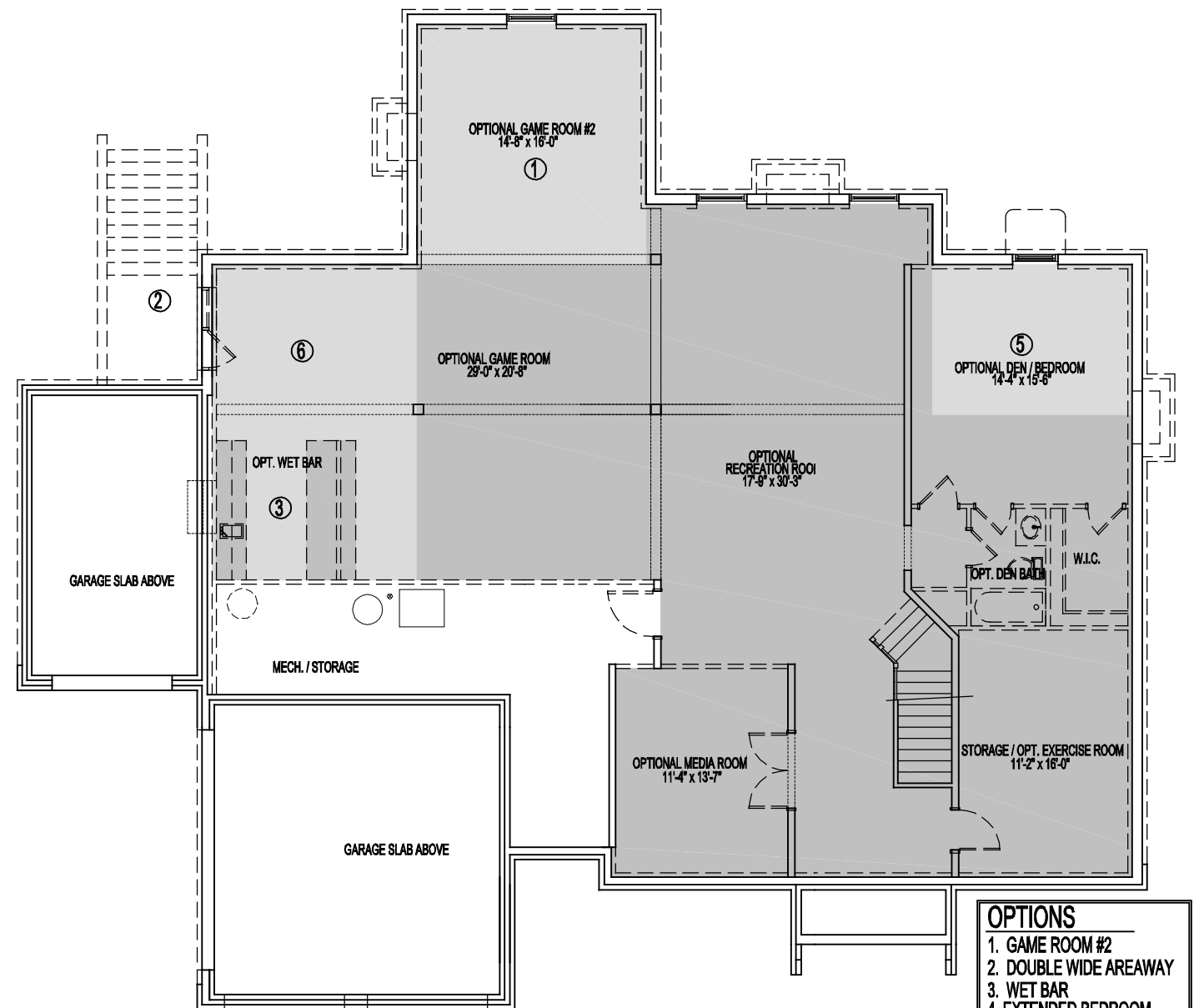
FOUNDATION / BASEMENT PLAN
