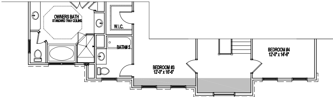
PARTIAL SECOND FLOOR PLAN ELEVATION 4A 01-13-20
