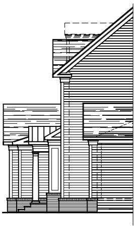
PARTIAL LEFT ELEVATION ELEVATION #1A 08-30-21
