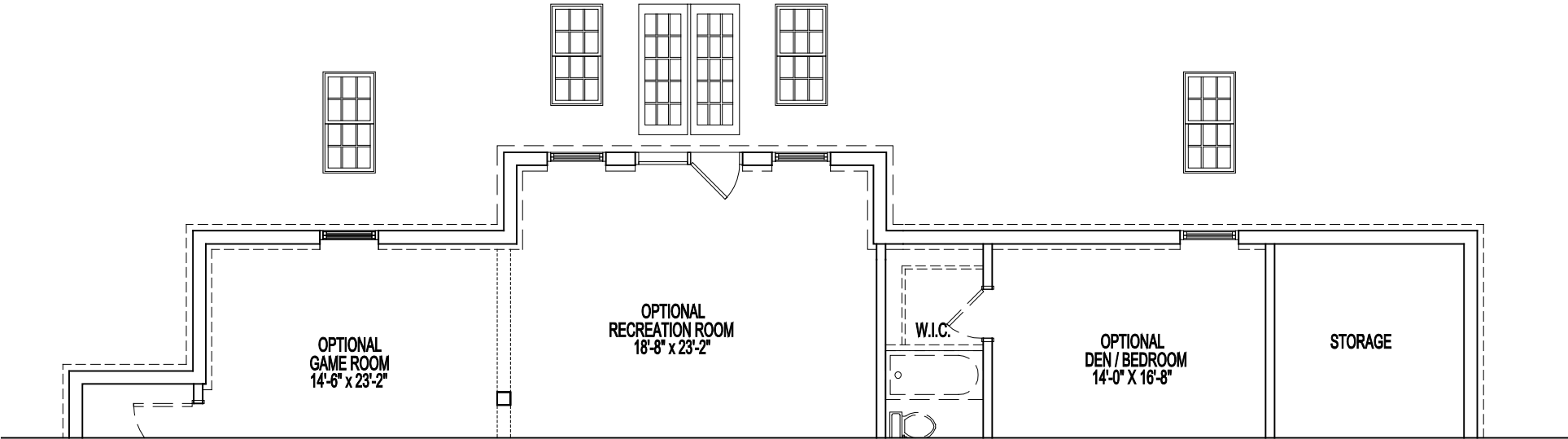
PARTIAL FOUNDATION / BASEMENT PLAN W/ WALKOUT 08-30-21
