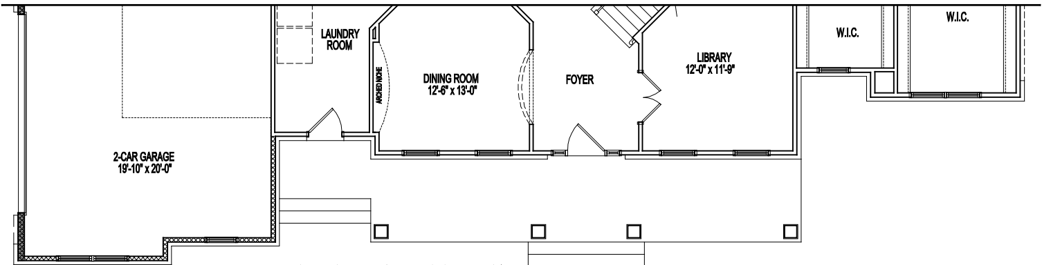
PARTIAL FIRST FLOOR PLAN ALTERNATE ELEVATION 1B 08-30-21
