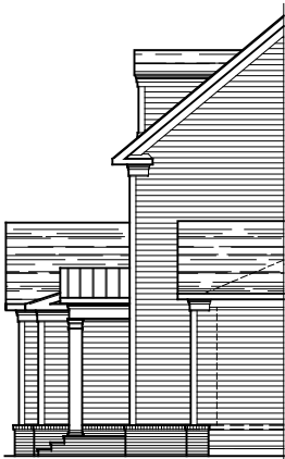
PARTIAL LEFT ELEVATION ALTERNATE ELEVATION #1A 08-30-21
