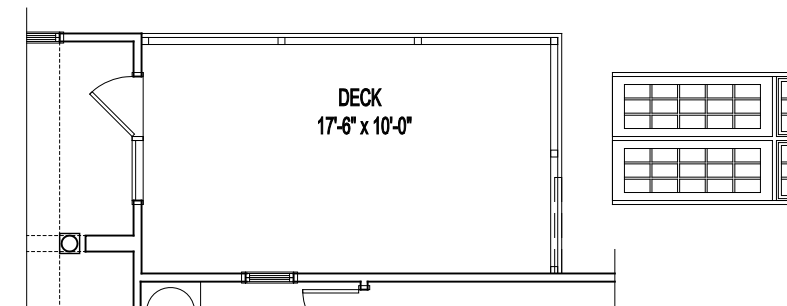
PARTIAL SECOND FLOOR PLAN
