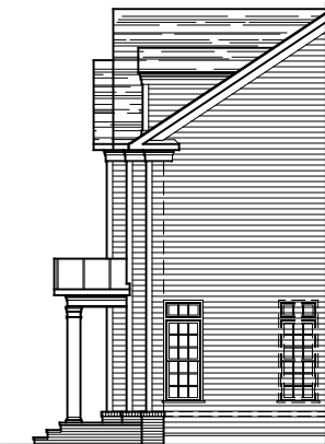
PARTIAL RIGHT SIDE ELEVATION ELEVATION #6A 02-11-21
