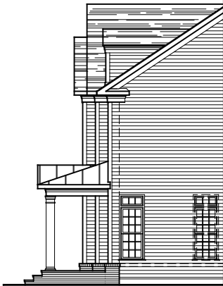
PARTIAL RIGHT SIDE ELEVATION ELEVATION #6B 02-11-21
