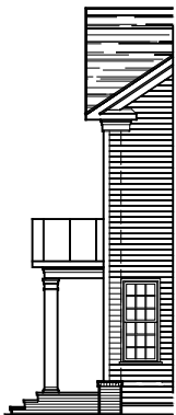
PARTIAL RIGHT SIDE ELEVATION ELEVATION #1A 02-11-21
