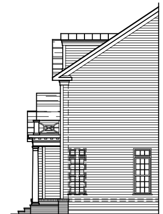
PARTIAL RIGHT SIDE ELEVATION ELEVATION #9B
