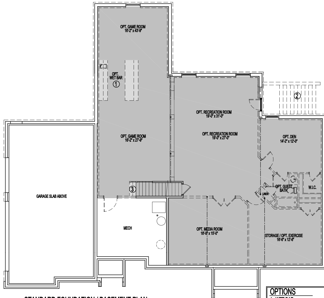
STANDARD FOUNDATION / BASEMENT PLAN
