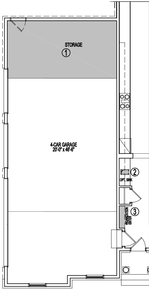
PARTIAL FIRST FLOOR PLAN
