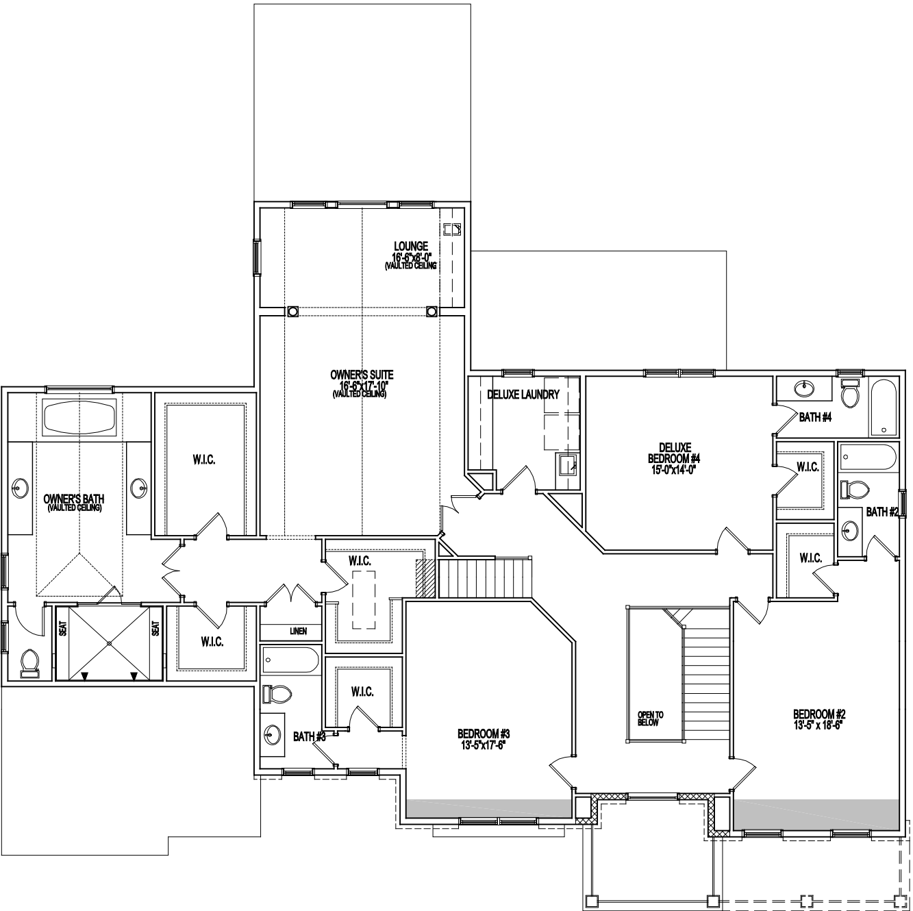
STANDARD SECOND FLOOR PLAN
