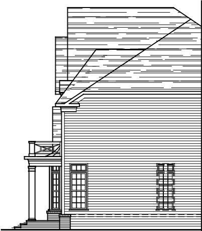
PARTIAL RIGHT SIDE ELEVATION ELEVATION #10A
