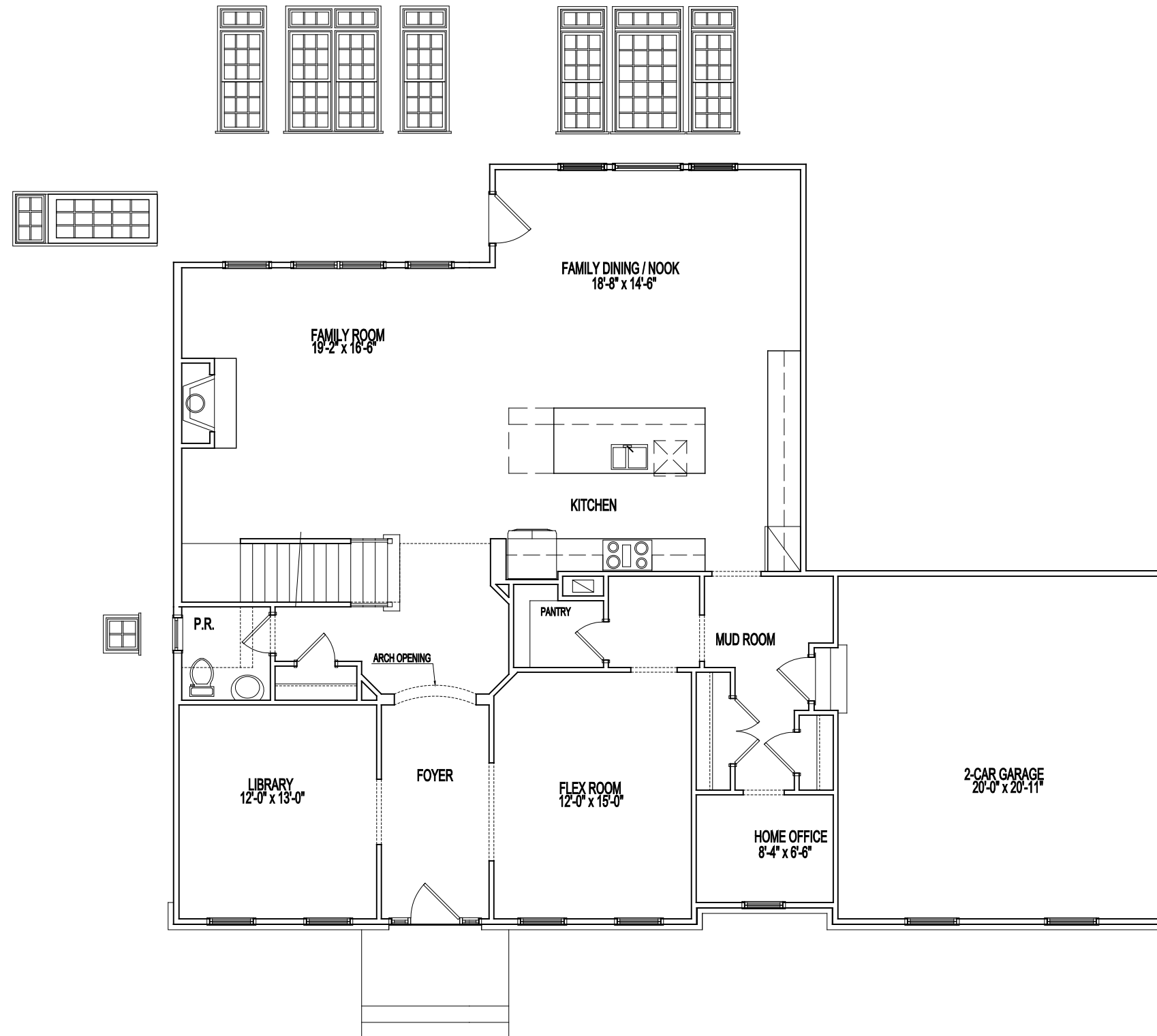
STANDARD FIRST FLOOR PLAN
