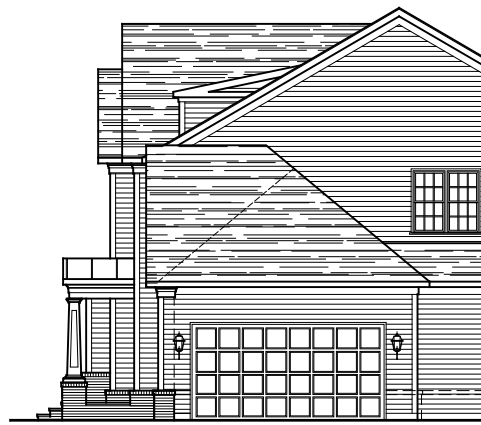
PARTIAL RIGHT SIDE ELEVATION ELEVATION #5A
