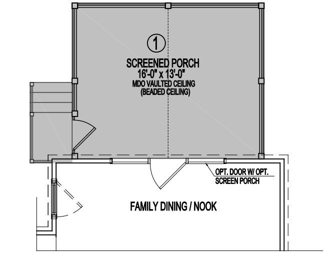
PARTIAL FIRST FLOOR PLAN 02-04-22
