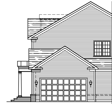
PARTIAL RIGHT SIDE ELEVATION ELEVATION #2A 02-04-22
