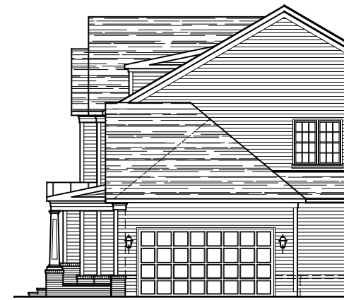
PARTIAL RIGHT SIDE ELEVATION ELEVATION #5B
