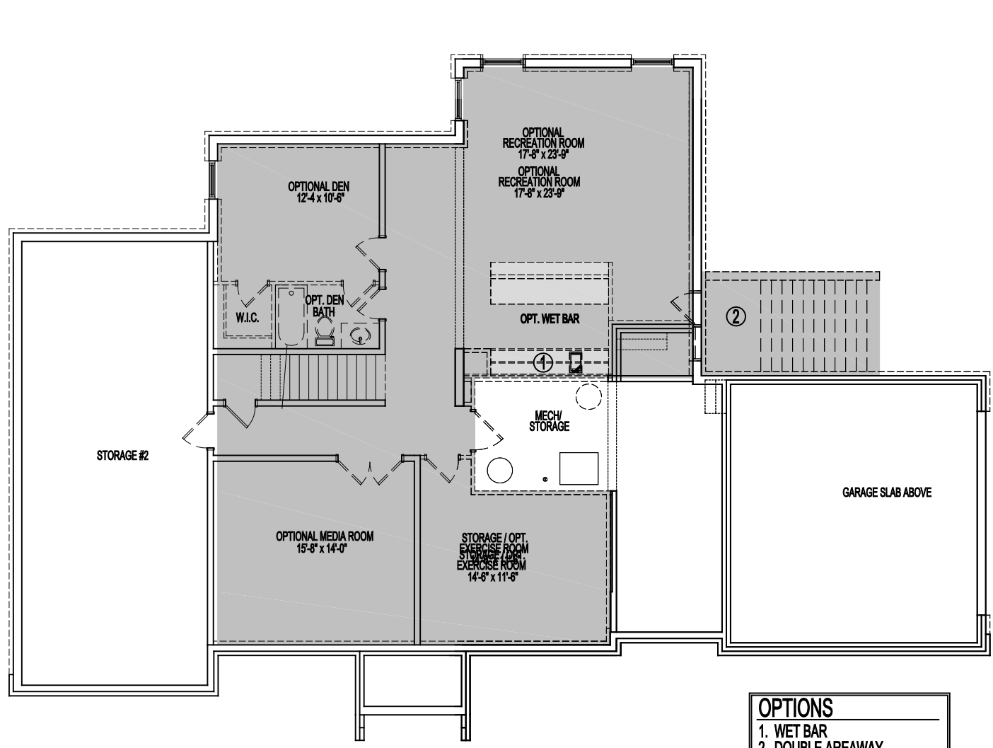
FOUNDATION / BASEMENT PLAN
