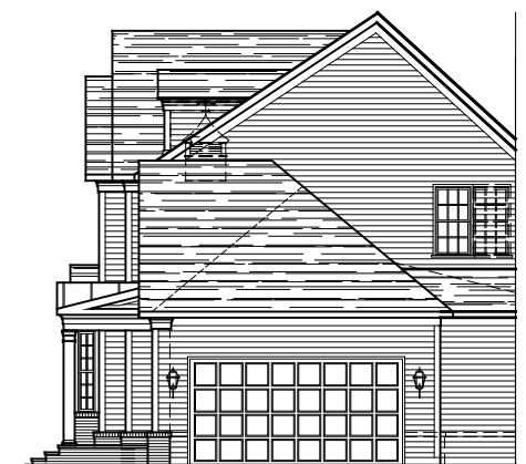
PARTIAL RIGHT SIDE ELEVATION ELEVATION #4B
