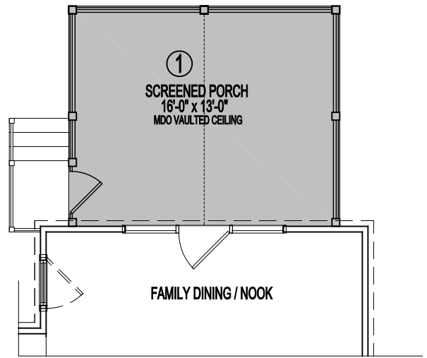
PARTIAL FIRST FLOOR PLAN 02-04-22
