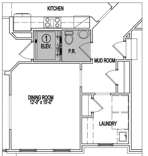
PARTIAL FIRST FLOOR PLAN 02-04-22
