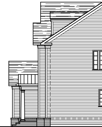
PARTIAL RIGHT ELEVATION ELEVATION #4A 04-04-2022
