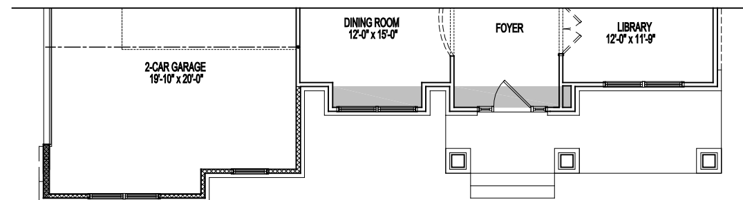
PARTIAL FIRST FLOOR PLAN ELEVATION #5B 04-04-2022
