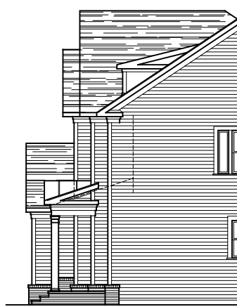
PARTIAL RIGHT ELEVATION ELEVATION #12A 04-04-2022
