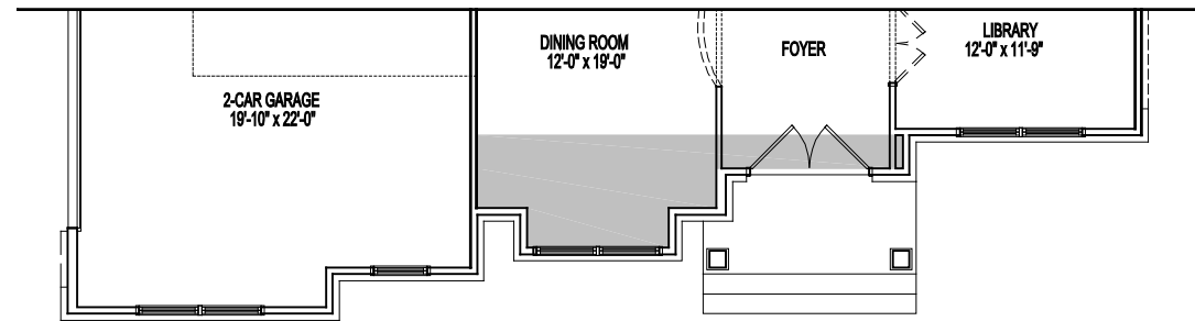
PARTIAL FIRST FLOOR PLAN ELEVATION #12A 04-04-2022
