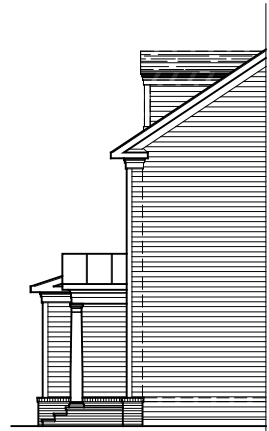
PARTIAL RIGHT ELEVATION ELEVATION #1A 04-04-2022
