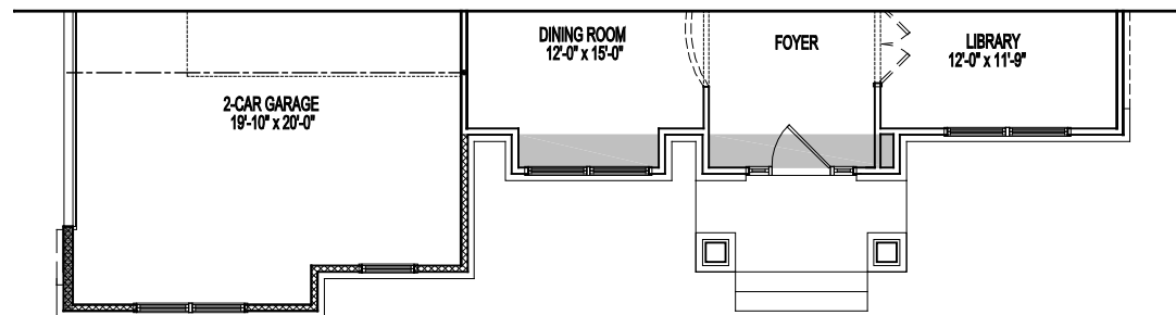
PARTIAL FIRST FLOOR PLAN ELEVATION #5A 04-04-2022
