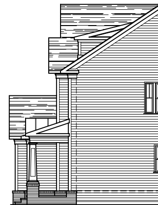
PARTIAL RIGHT ELEVATION ELEVATION #5B 04-04-2022
