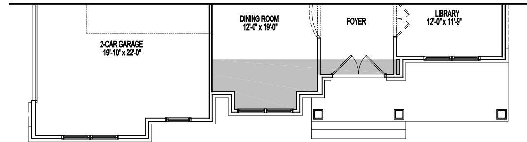
PARTIAL FIRST FLOOR PLAN ELEVATION #12B 04-04-2022
