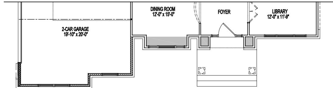
PARTIAL FIRST FLOOR PLAN ELEVATION #4 & 4A 04-04-2022
