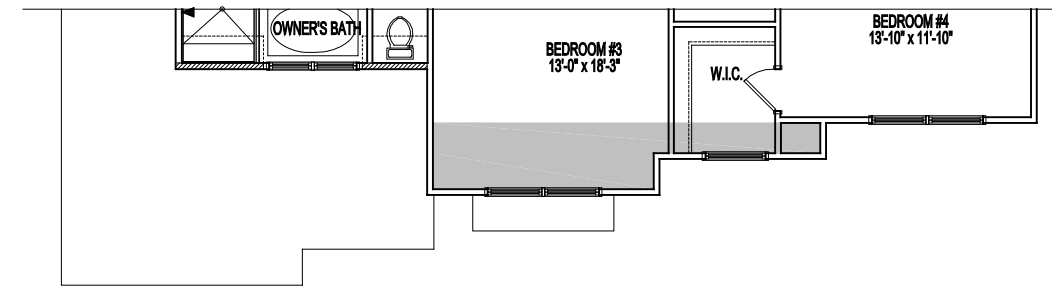
PARTIAL SECOND FLOOR PLAN ELEVATION #12A & #12B 04-04-2022
