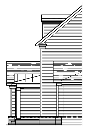
PARTIAL LEFT ELEVATION ALTERNATE ELEVATION #1B 04-08-22
