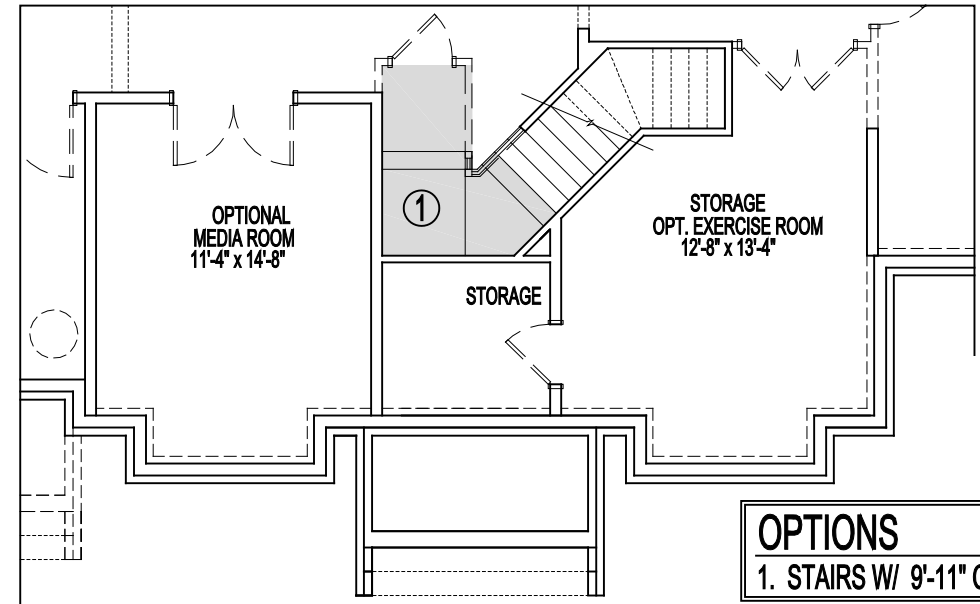
FOUNDATION / BASEMENT PLAN
