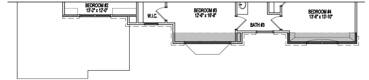
PARTIAL SECOND FLOOR PLAN ELEVATION 6A 04-08-22
