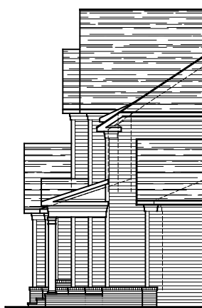
PARTIAL LEFT ELEVATION ELEVATION #8B 04-08
