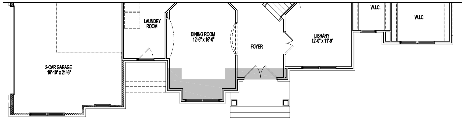
PARTIAL FIRST FLOOR PLAN ELEVATION 8A 04-08-22
