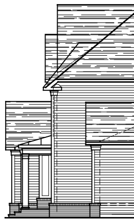
PARTIAL LEFT ELEVATION ELEVATION #6A 04-08-22
