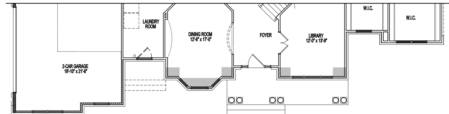
PARTIAL FIRST FLOOR PLAN ELEVATION 7B 04-08-22
