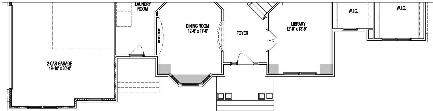
PARTIAL FIRST FLOOR PLAN ELEVATION 6A 04-08-22
