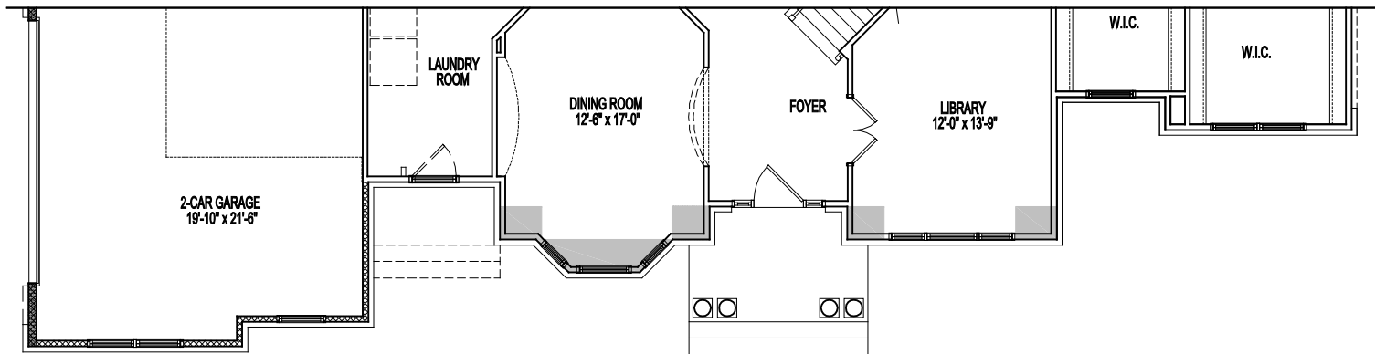
PARTIAL FIRST FLOOR PLAN ELEVATION 7A 04-08-22
