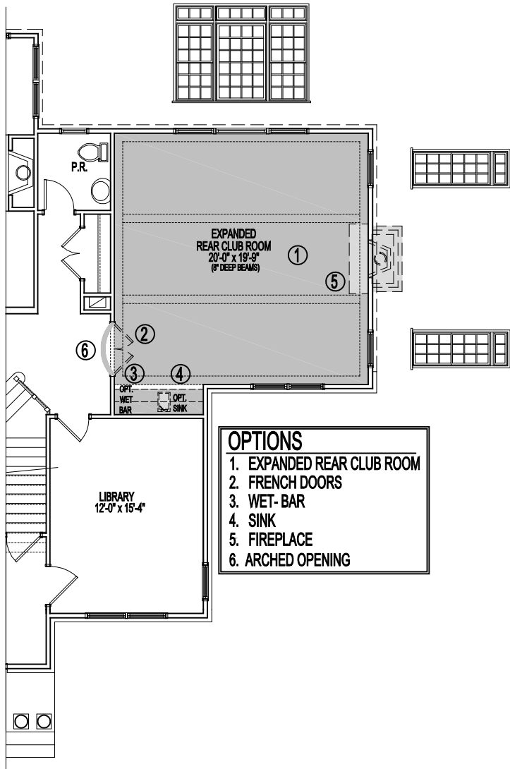
PARTIAL FIRST FLOOR PLAN 10-03-22
