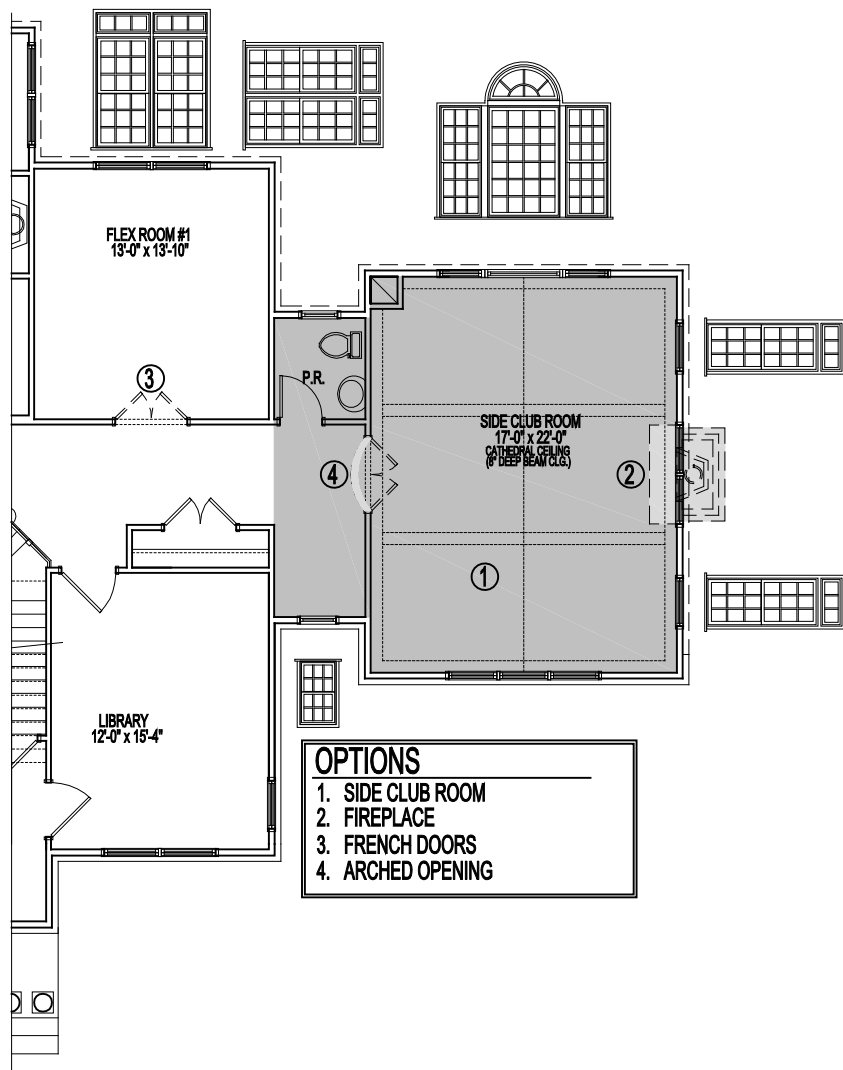
PARTIAL FIRST FLOOR PLAN 10-03-22
