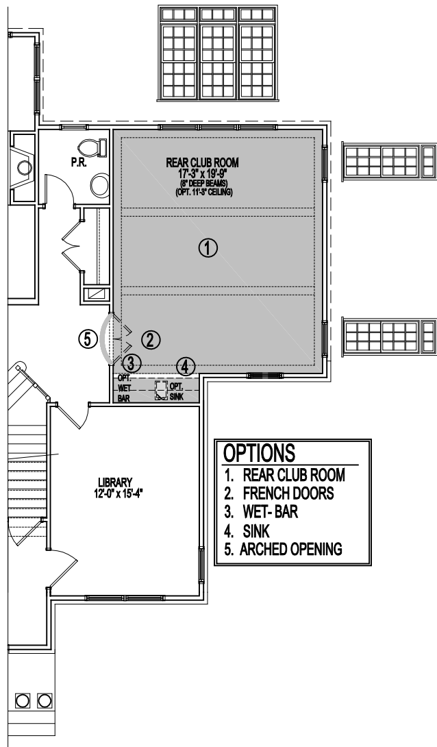
PARTIAL FIRST FLOOR PLAN 10-03-22
