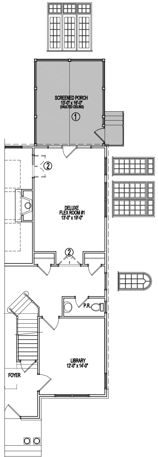
PARTIAL FIRST FLOOR PLAN
