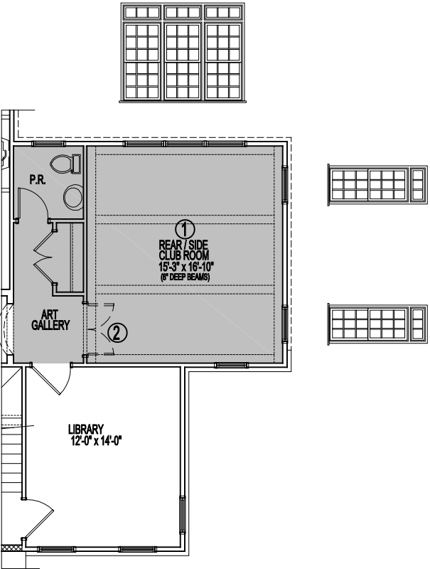
PARTIAL FIRST FLOOR PLAN 08-22-22
