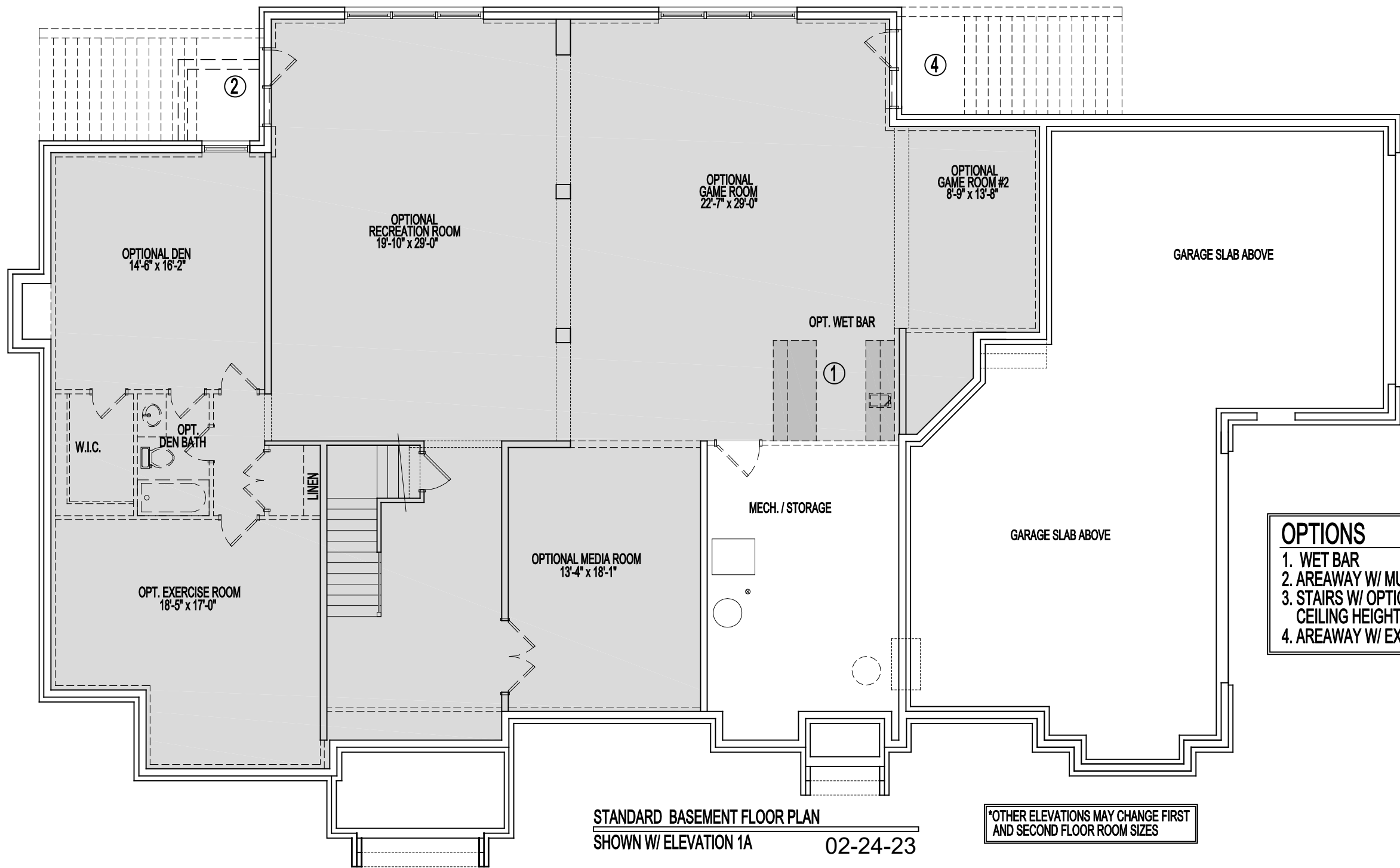
FOUNDATION / BASEMENT PLAN
