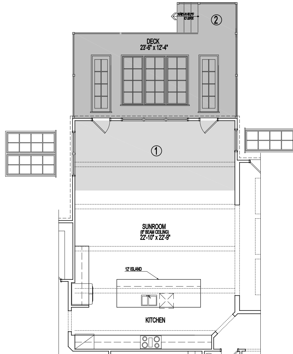
PARTIAL FIRST FLOOR PLAN
