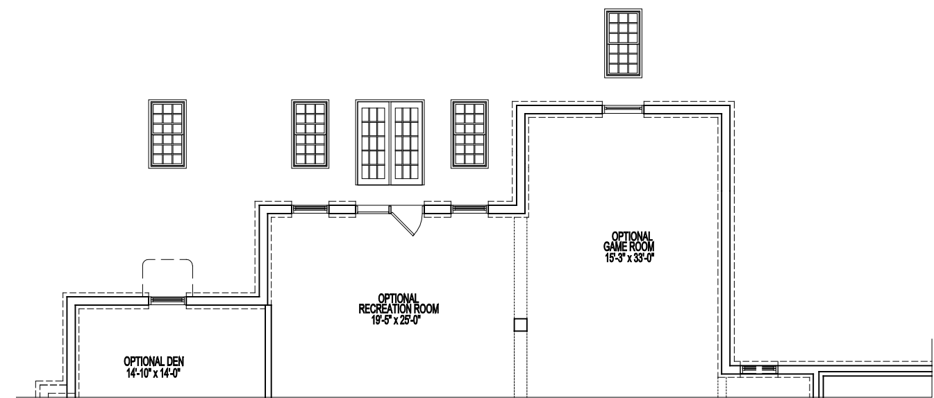
PARTIAL BASEMENT FLOOR PLAN WITH WALKOUT
