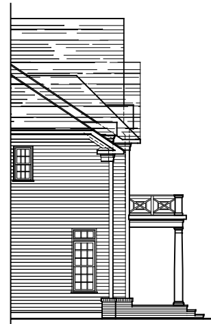
PARTIAL LEFT SIDE ELEVATION ELEVATION #5B 03-29-23
