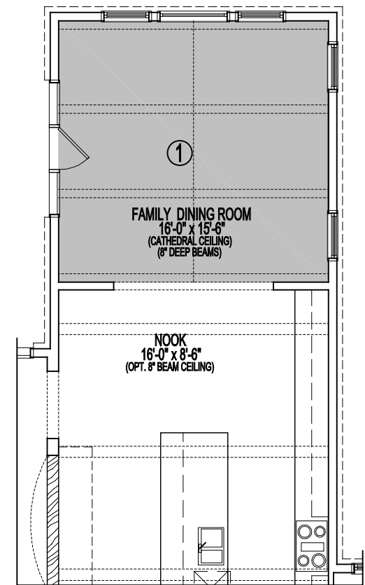
PARTIAL FIRST FLOOR PLAN 03-29-23
